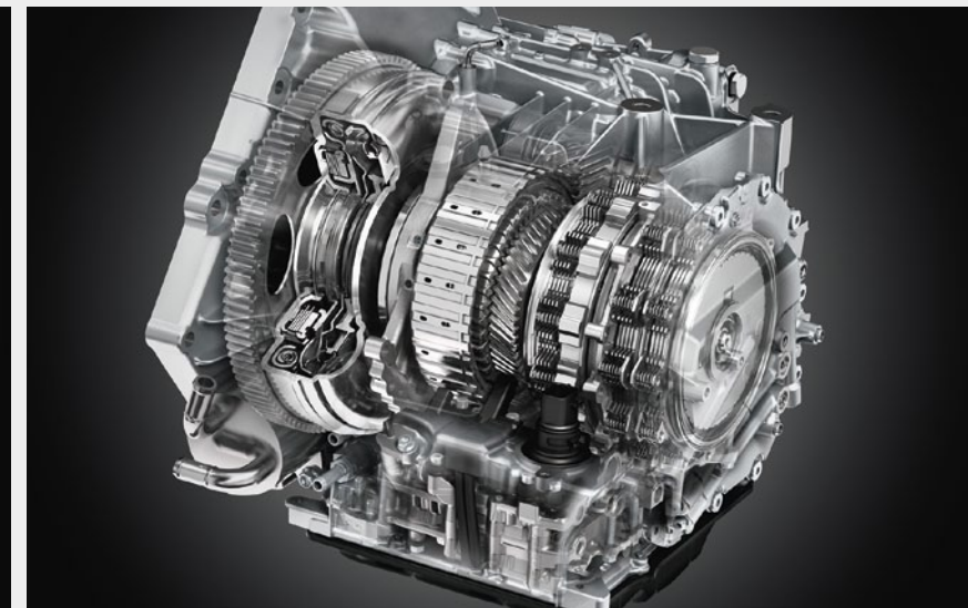
TRANSMISSIONS SKYACTIV-MT ET SKYACTIV-DRIVE
