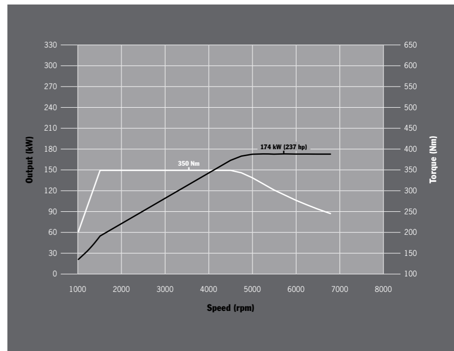
Macan: 350 Nm at 1,500–4,500 rpm, 174 kW (237 hp) at 5,000–6,800 rpm
